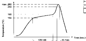
Soldering profile MMS 1010 D-R
